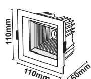
Dimension ( mm )
